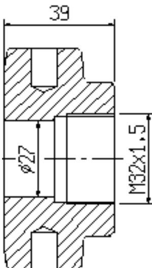
Ecrou type 341-10-223
